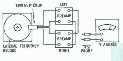
Fig. 1. Checking phase with a VU meter.
