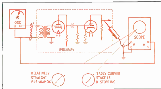
Fig. 4. Check for distortion in low-level stage.
