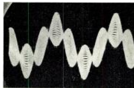
Fig. 7. Subchannel only, 45° out of phase; pilot synchronized method of monitoring.
