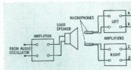
Fig. 3. Setup for checking microphone phase with an audio oscillator and scope.
