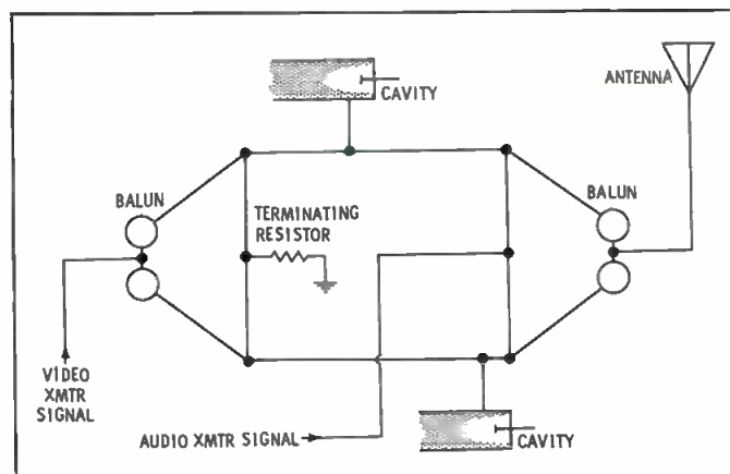
Fig. 2. Basic schematic of notch diplexer.
